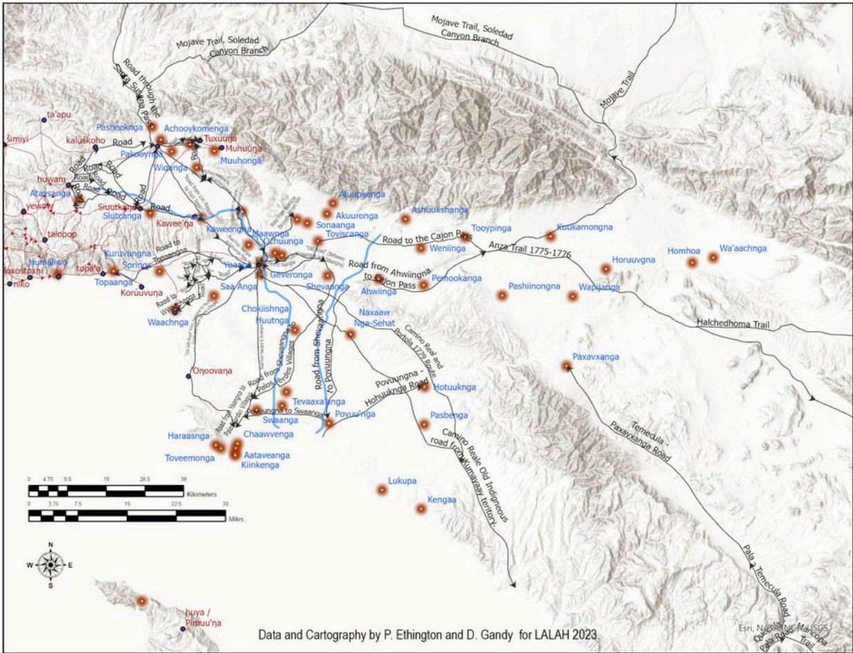
Figure 0-2. Indigenous roads and pathways within and extending from the Los Angeles Basin.
