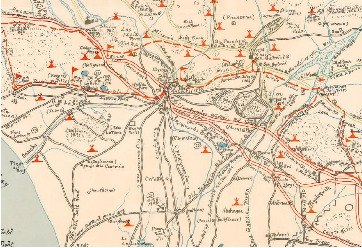
Figure 6-8. The Kirkman-Harriman Map of 1938 (Detail).
